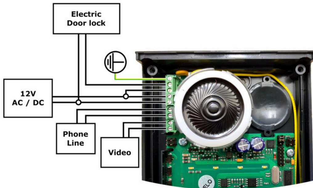
Fig.: Lock Connection
