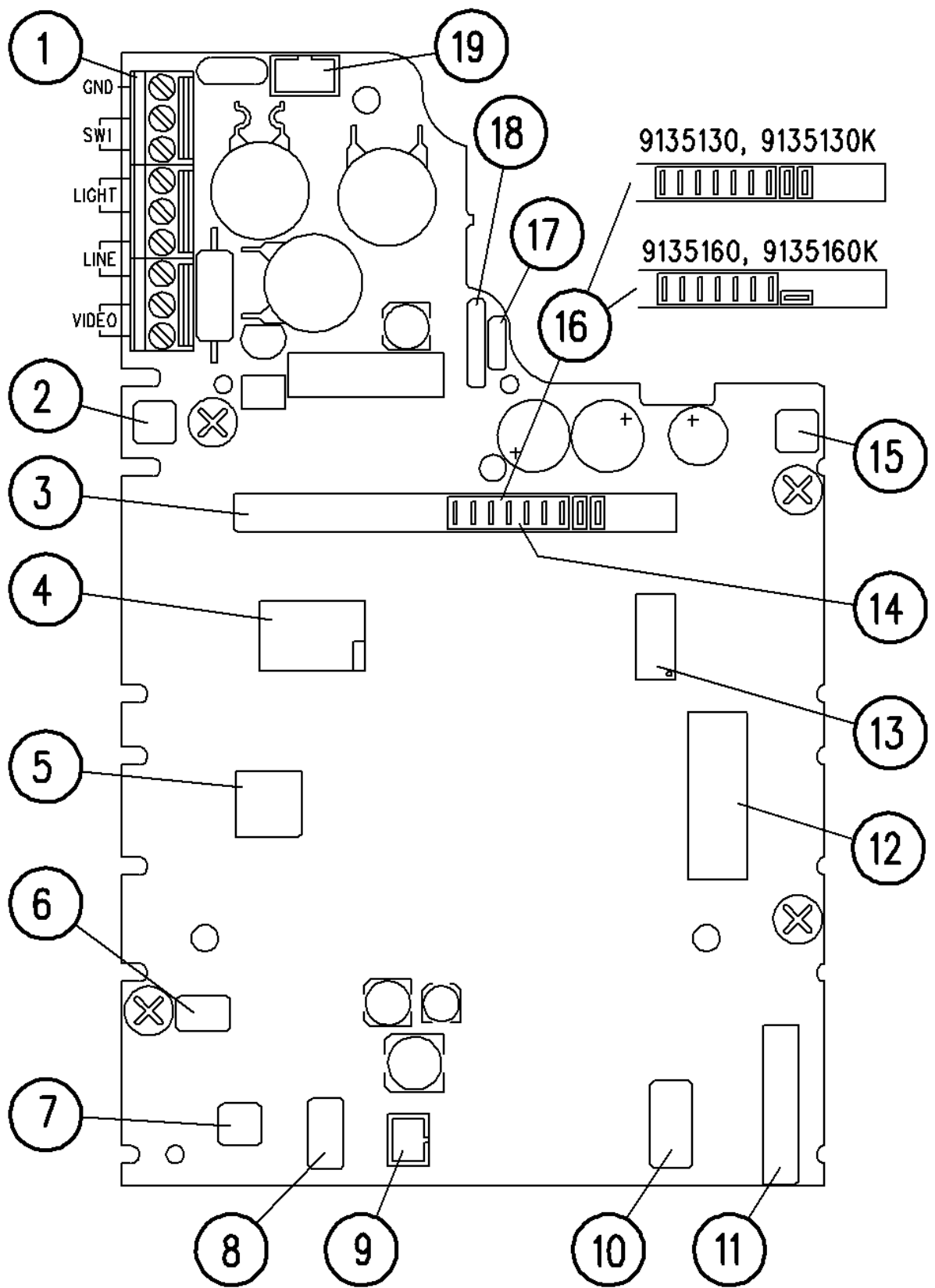
Fig.: PCB Layout, Version 10
