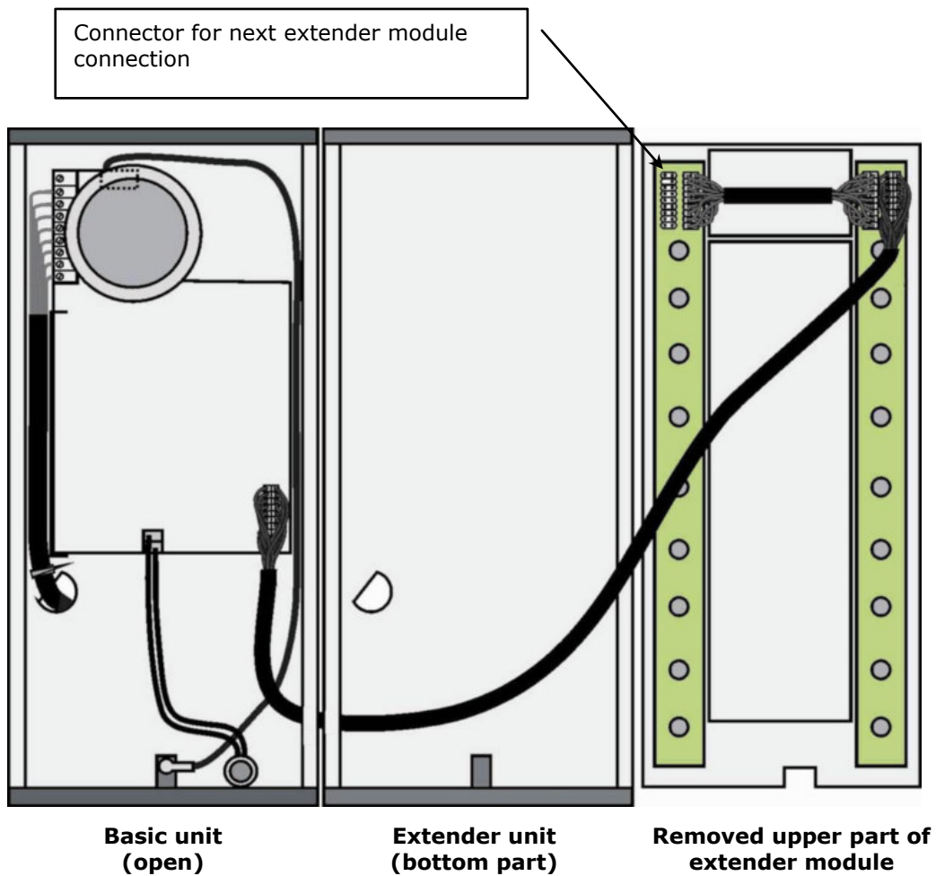
Fig.: 16-Button Extender Module Connection to Basic Unit
