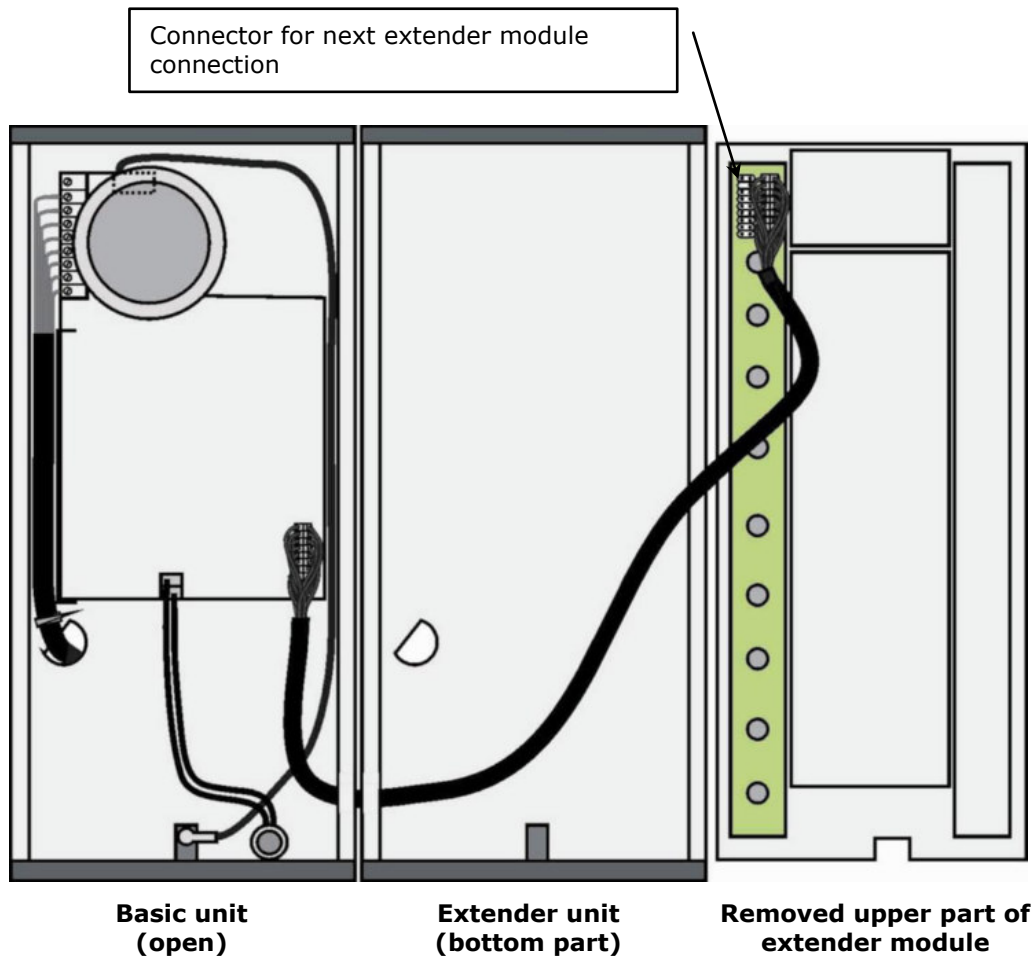
Fig.: 8-Button Extender Module Connection to Basic Unit
