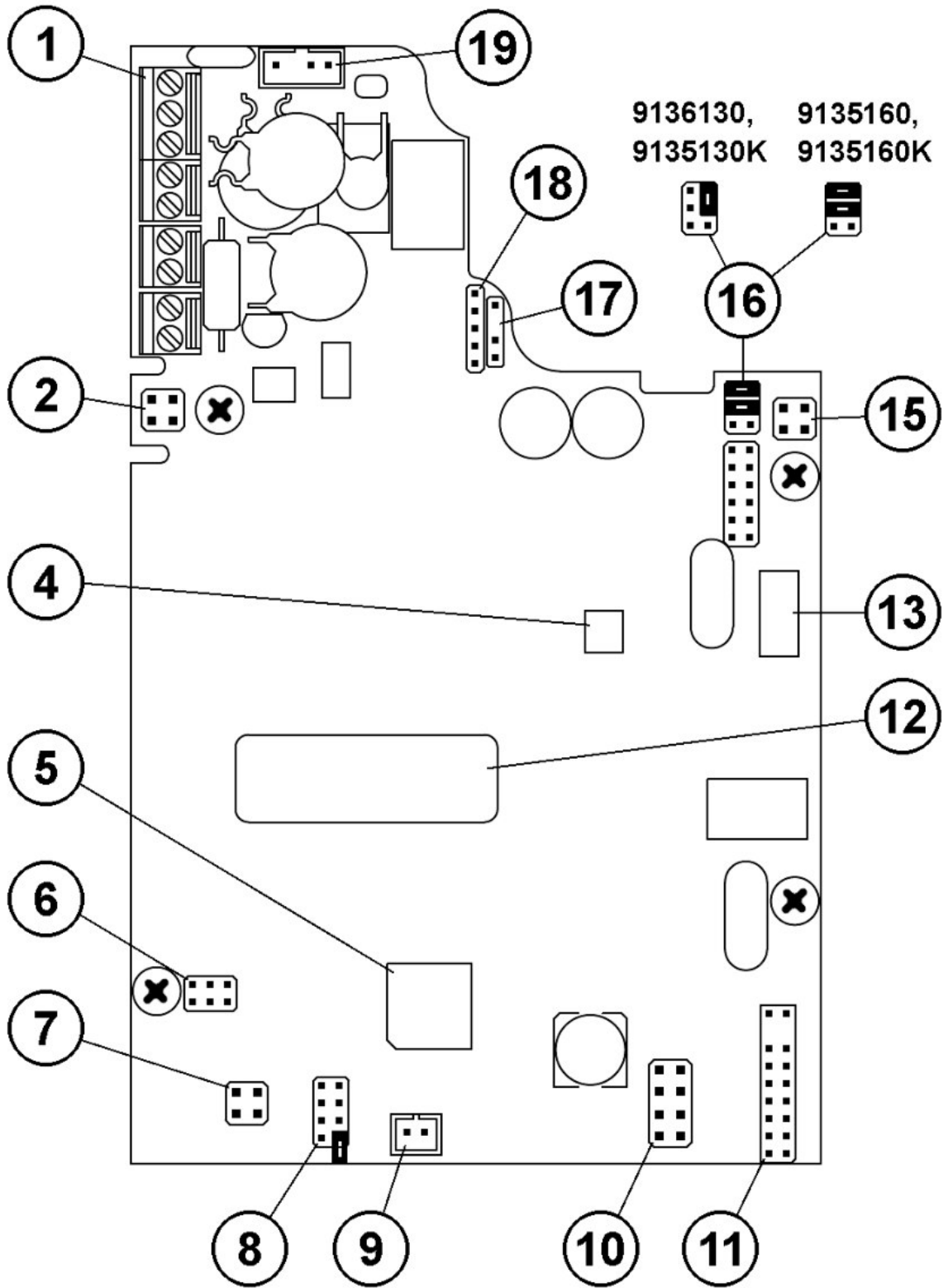
Fig.: PCB Layout, Version 14
